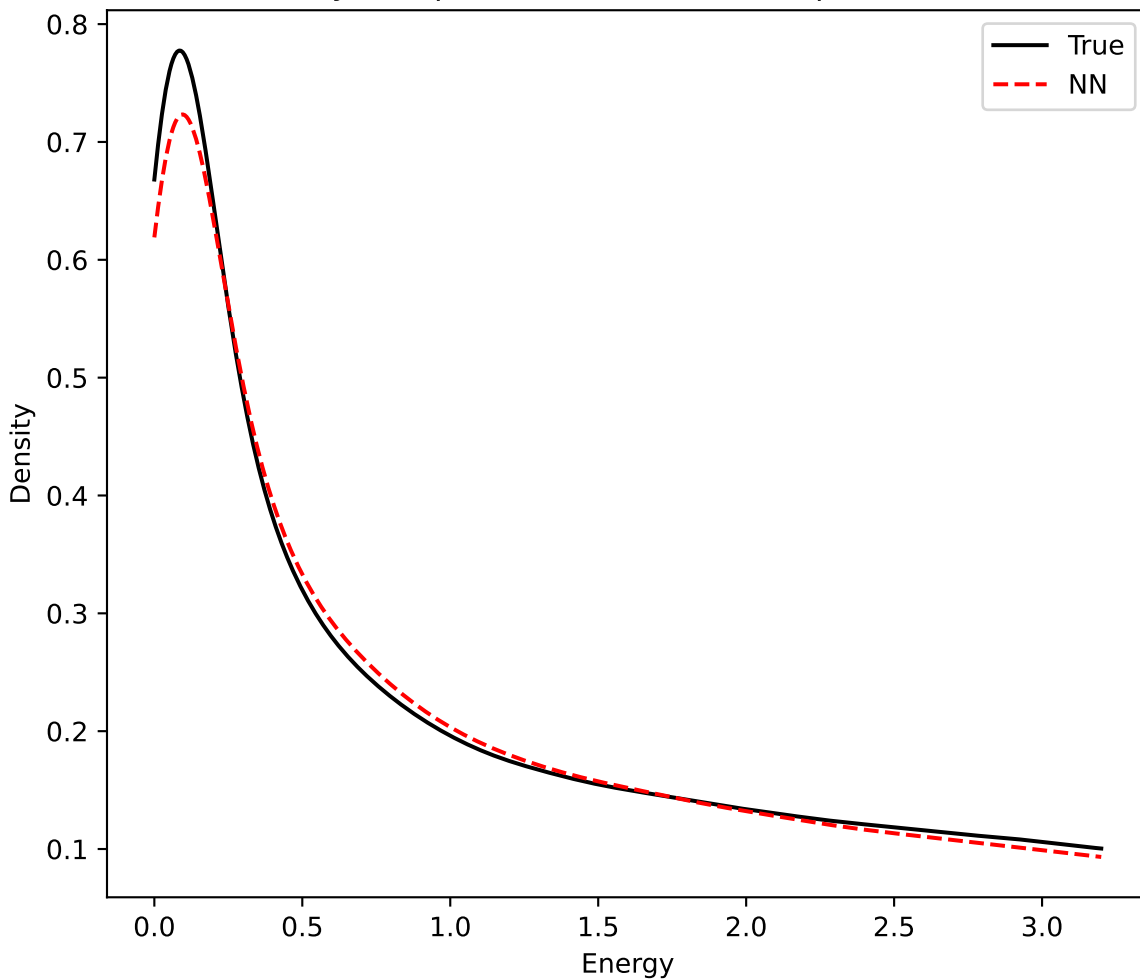
TKE Density Comparison with KS: 0.017, p-value: 1.3e-100
