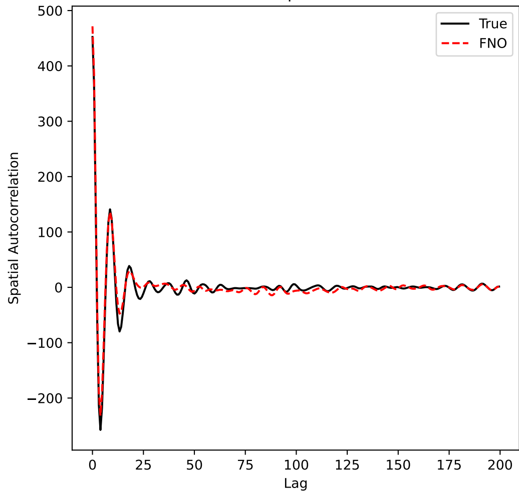
Autocorrelation Comparison with MSE = 63
