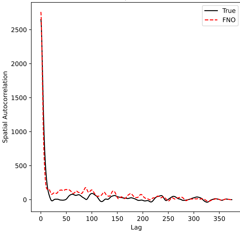
Autocorrelation Comparison with MSE = 5e+03
